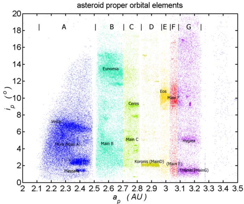
Figure 7: This plot highlights some of the major families or groups in the asteroid belt. Vesta (group A) and Ceres (group C) are labeled on the plot. Asteroid proper orbital elements (n.d.). Source: http://en.wikipedia.org/wiki/File:AsteroidIncAu.png (made available under a Creative Commons License).
