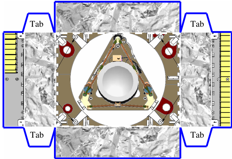
Aft Structure Assembly
